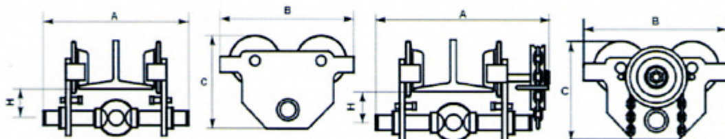
PUSH TROLLEY
